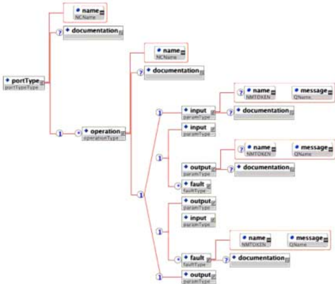
Figure 2.6 <portType> element structure.
