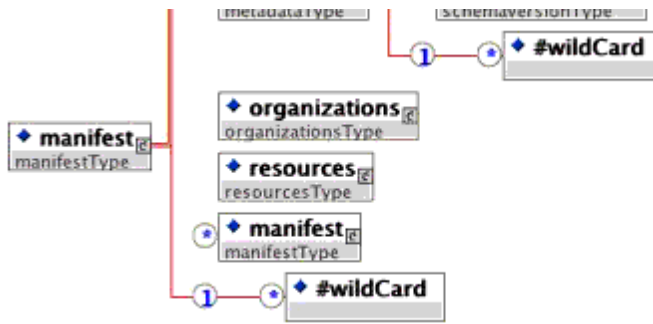
Figure 3.2 <metadata> elements.
