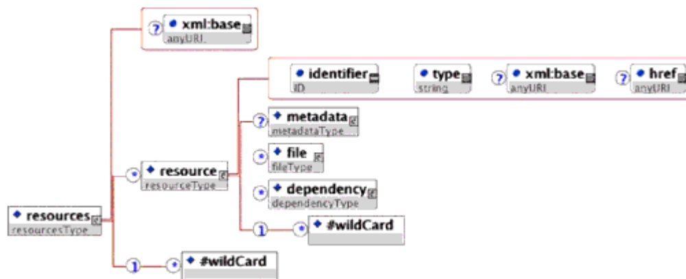
Figure 3.4 - <resources> elements.
