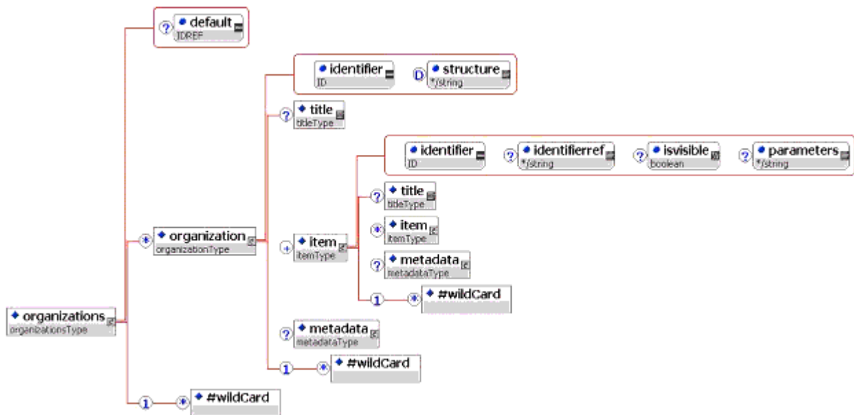
Figure 3.3 - <organizations> elements.
