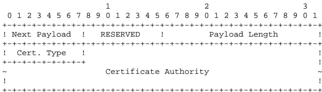
Figure 11: Certificate Request Payload Format
