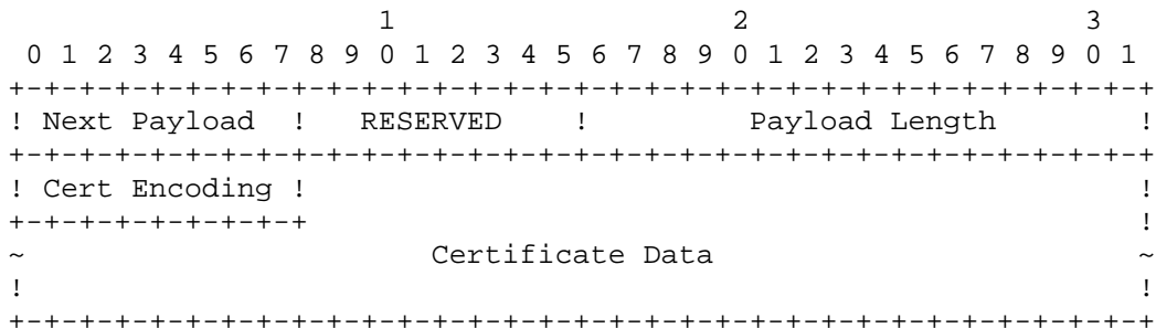
Figure 10: Certificate Payload Format
