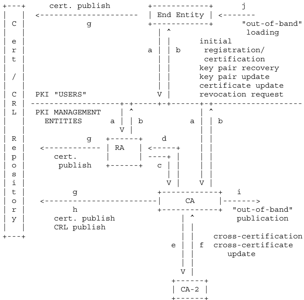
Figure 1 - PKI Entities
